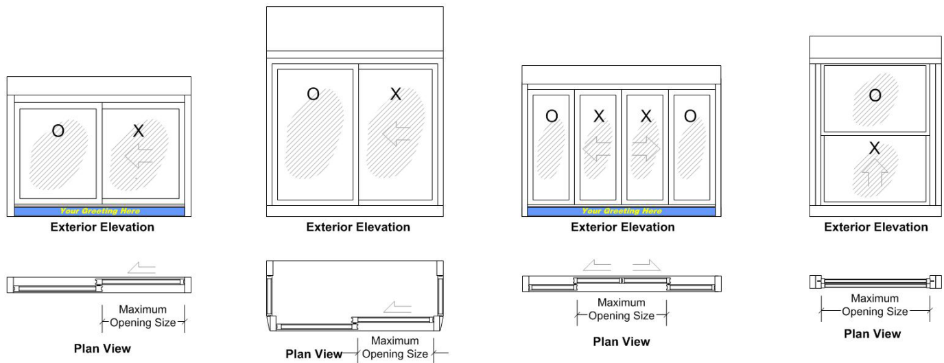
SS Series In-Line Side Slider
