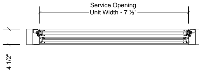
PLAN VIEW
