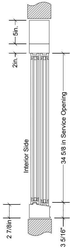
SECTION
