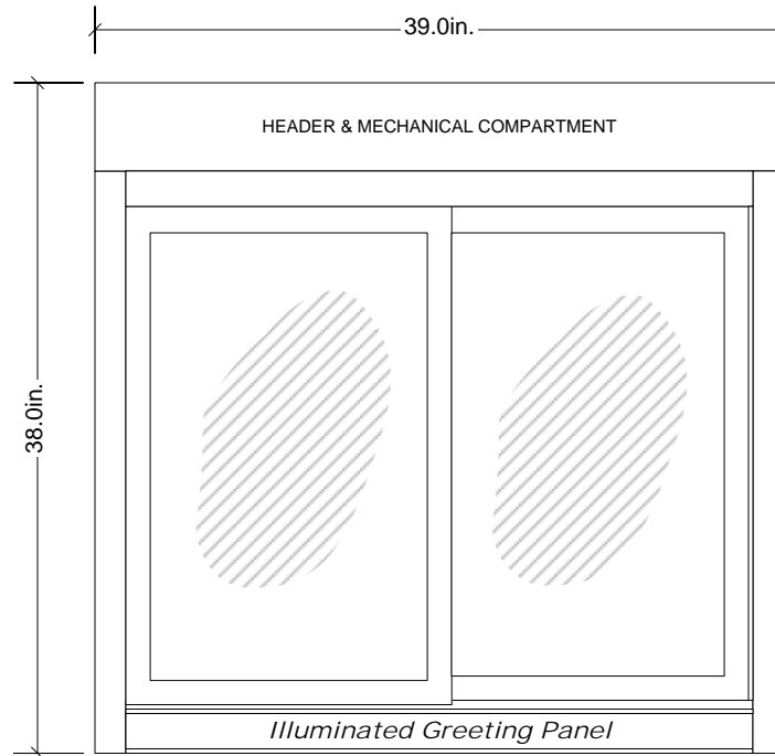
EXTERIOR ELEVATION
