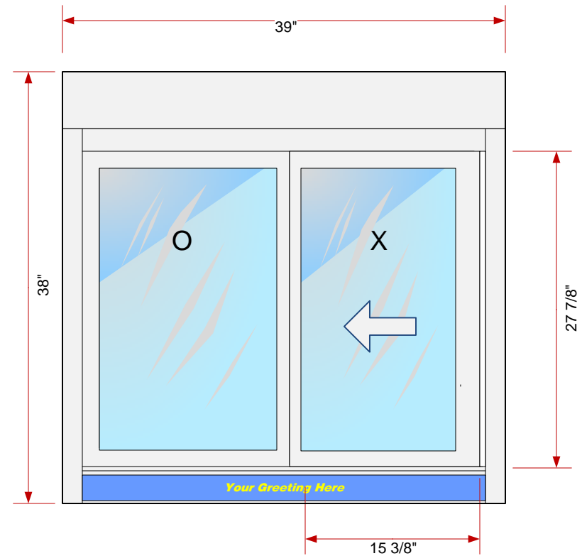
EXTERIOR ELEVATION
