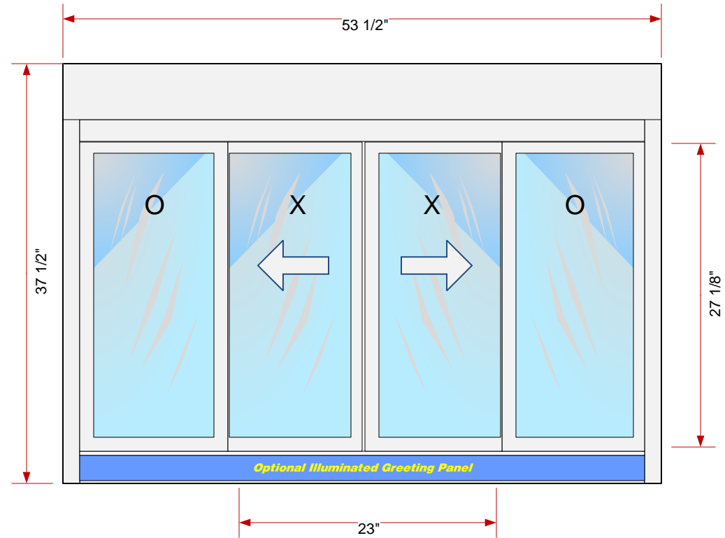
EXTERIOR ELEVATION
