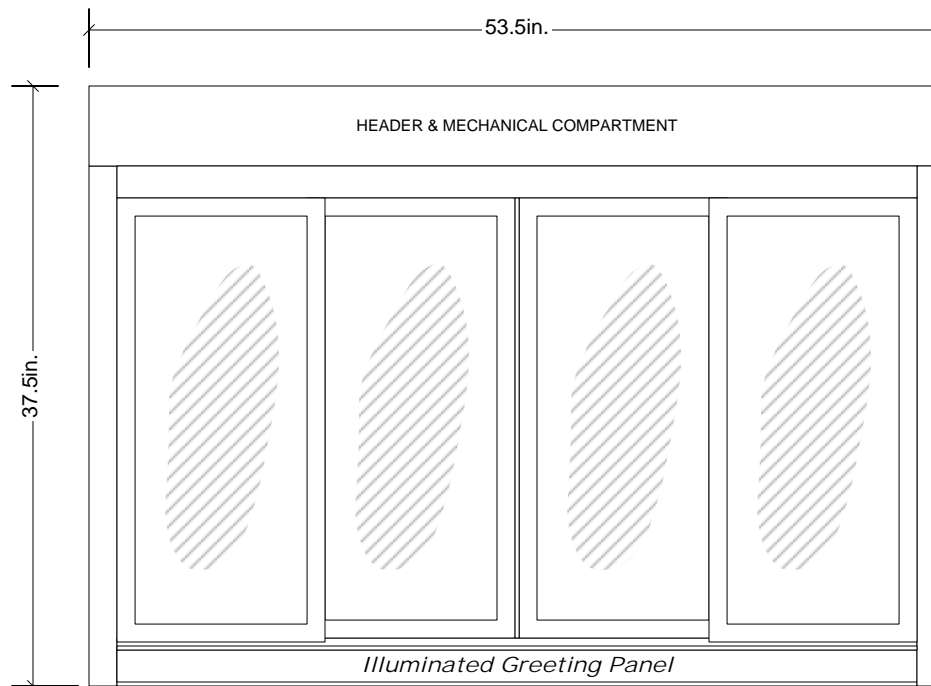
EXTERIOR ELEVATION
