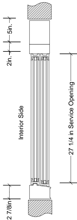
SECTION
