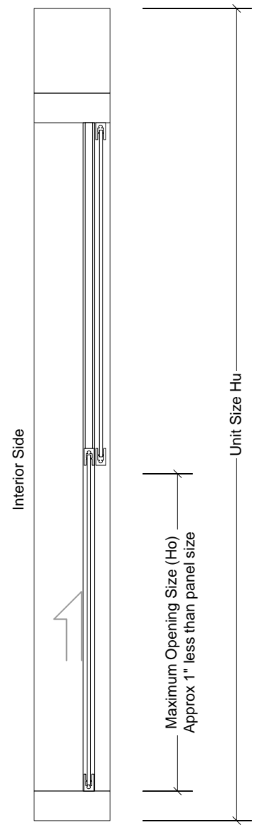
Section View
